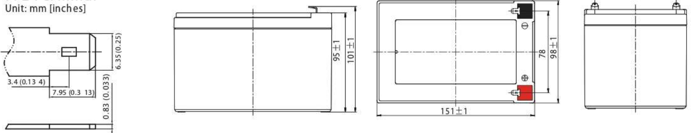
T1 2 Terminal Unit: mm [inches]
